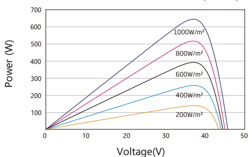
P-V CURVES OF PV MODULE(645W)
