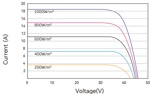
I-V CURVES OF PV MODULE(675 W)
