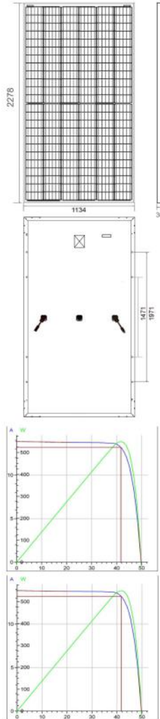
Dimension of PV Modules Unit: mm
