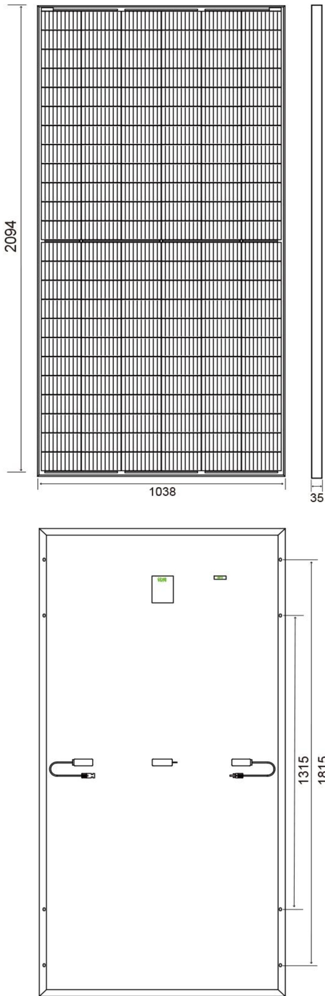
Dimension of PV Modules Unit: mm
